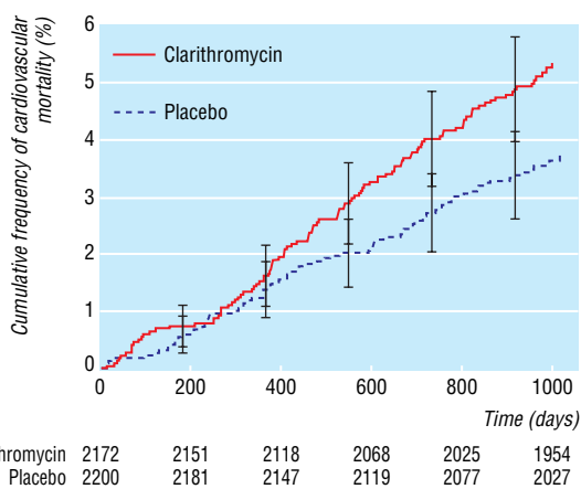
Fig 3 Kaplan-Meier estimate (with 95% confidence intervals) of cardiovascular mortality according to intervention. Figures below the diagram are biannual number at risk in the clarithromycin and placebo groups
