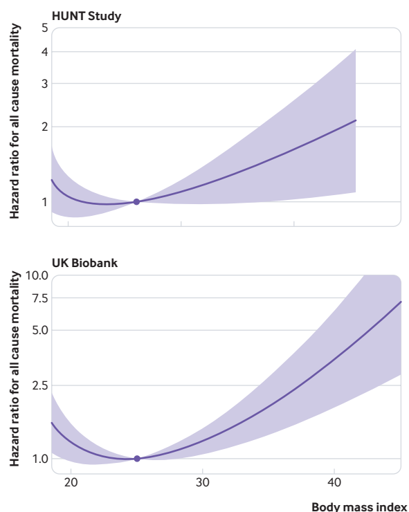
Fig 2 | Non-linear mendelian randomisation. Dose-response curve between body mass index and all cause mortality for HUNT Study and UK Biobank. Gradient at each point of the curve is the localised average causal effect. Shaded areas represent 95% confidence intervals
