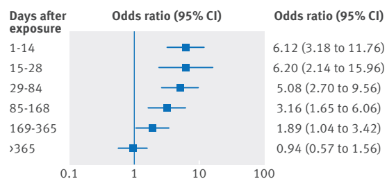
Fig 4 | Individual crude multilevel odds ratios for trimethoprim resistance in urinary isolates of children from Duffy and colleagues 24 and previous trimethoprim prescribing
