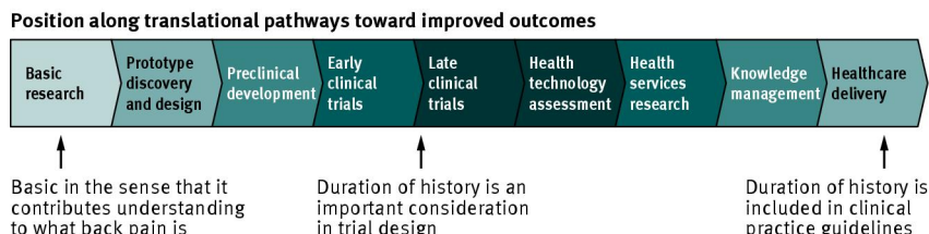
Fig 4 Example of use of fundamental prognosis research to define clinically relevant subgroups: duration of low back pain at presentation (<3 or ≥3 years) and the time to improvement of disability disease (drawn using data from Dunn et al 46 ). Path element adapted from chart 7.1 in the Cooksey report (2006) http://bit.ly/Ro27rL (made available for use through the Open Government License)
