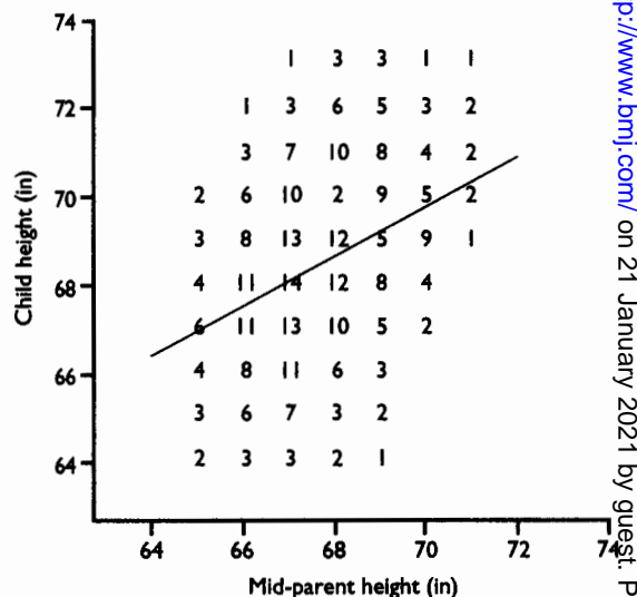
Galton's original data showing the relation between the heights of children and their parents, with regression line
