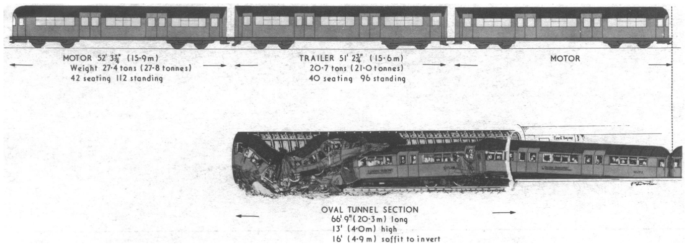
FIG. 1—Scene of Moorgate tube disaster and details of train.
